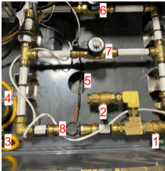
Figure 6) Plumbing Layout in the Base of the Watering System
