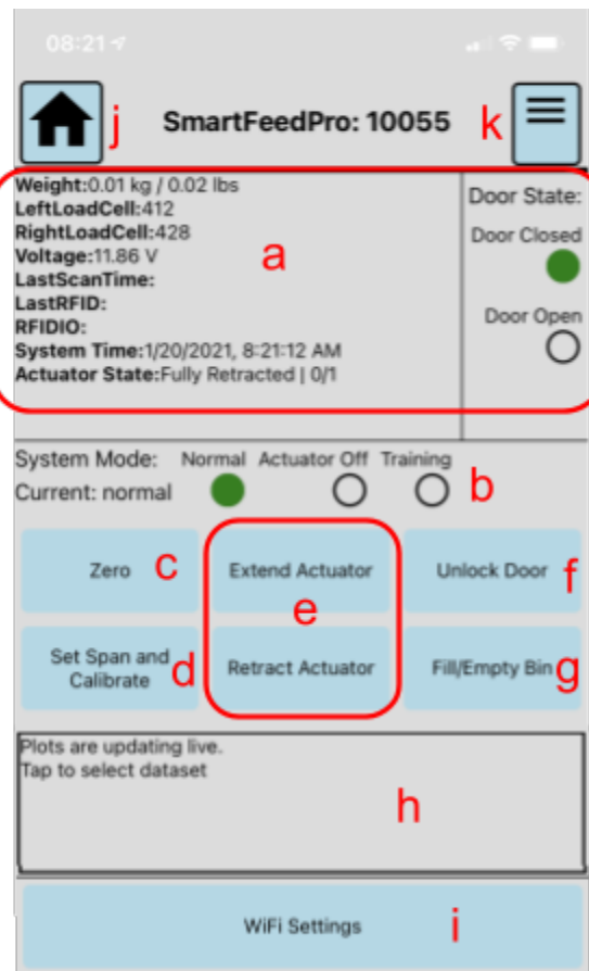
Figure 24) Control Feed Main Interface Controls
