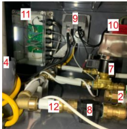
Figure 6) Plumbing Layout in the Base of the Watering System
